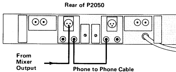
Fig. 40A — “Chaining” of Inputs for Mono Operation into Two 8\Omega Loads.
