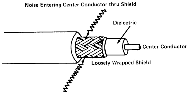
Fig. 47 – Poor Quality Shielded Cable
