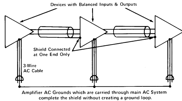
Fig. 49 – Telescoping Shield
