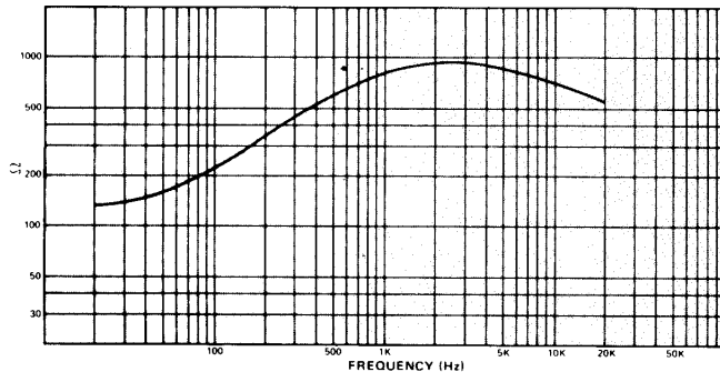
Fig. 45 — Impedance of Poor Quality 70-Volt Speaker Transformer (Connected to 8\Omega Speaker, Tapped for "5 Watts," looking into Primary). 25-Volt Transformers Exhibit Similar Behavior.
