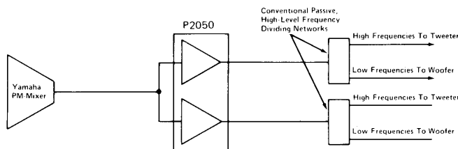
Fig. 57A – System using Conventional, Passive/High-Level Frequency Dividing Networks.
