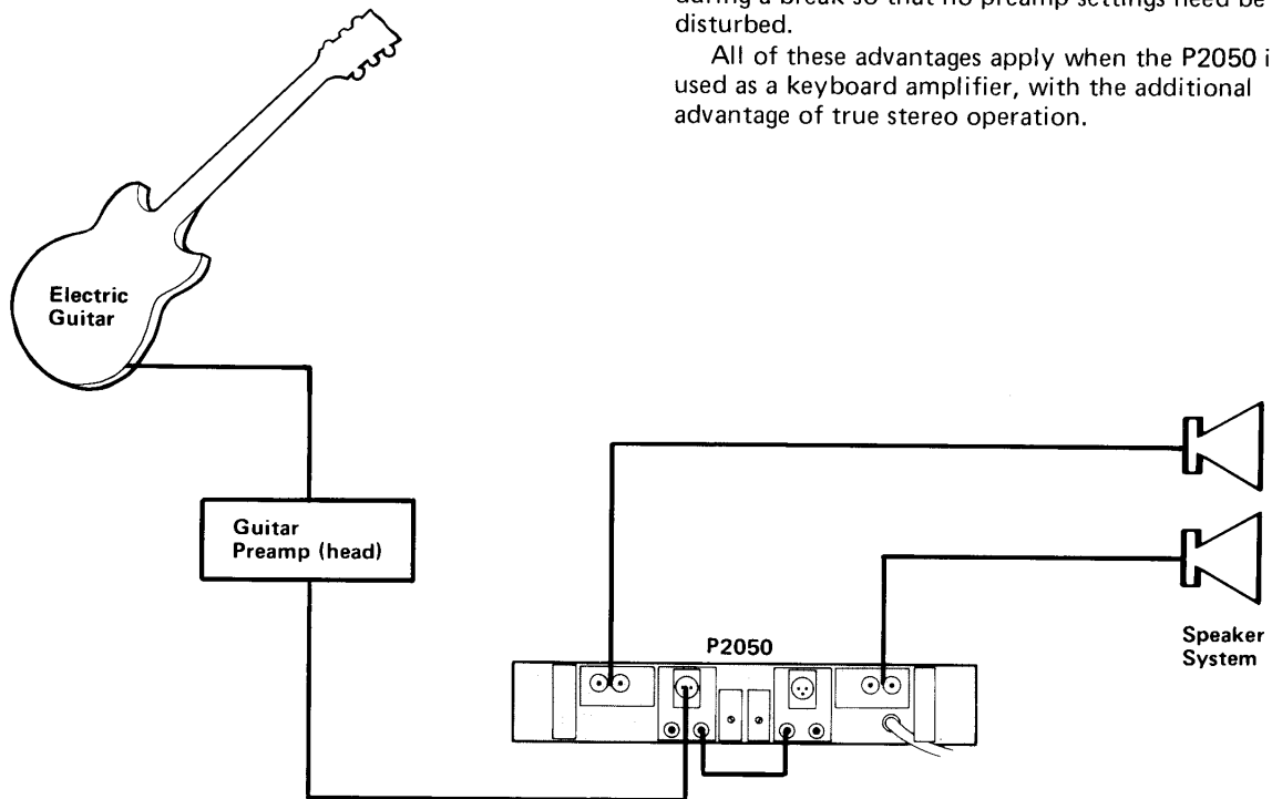
Fig. 67 – Instrument Amplifier
